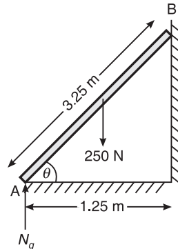
Figure 8.67 Example 8.21.
