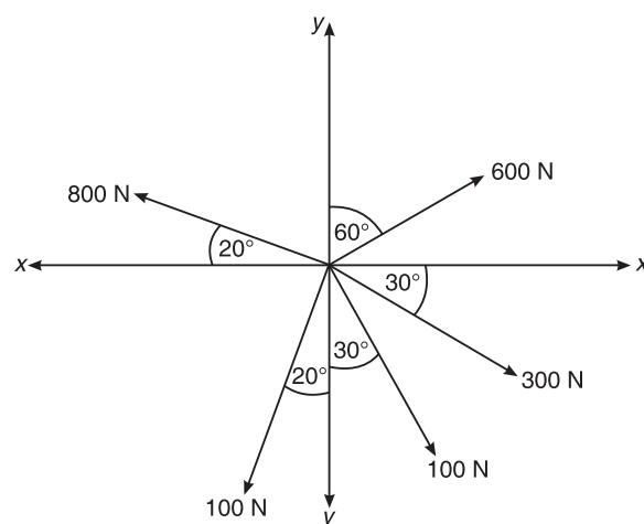
Figure 3.5 Example 3.5.
