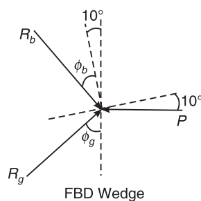
FBD Wedge
