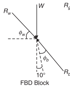
FBD Block
