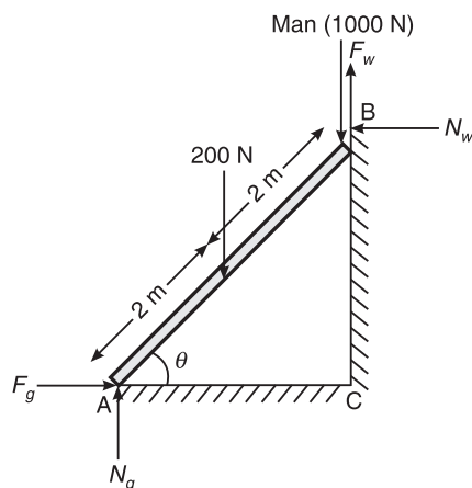
Figure 8.75 Example 8.24.
