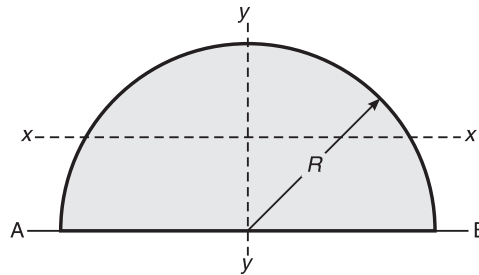
Figure 10.9 Semicircular lamina.
