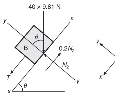
Figure 8.47 Example 8.15.
