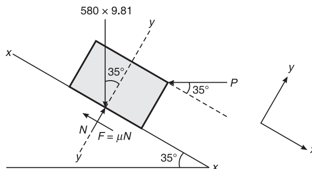
Figure 8.21 Example 8.7.
