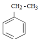
Ethylbenzene (Ethyle Benzol)
