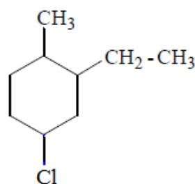
4 - Chloro - 2 - ethyl - 1 - methyl Cyclo Hexane
