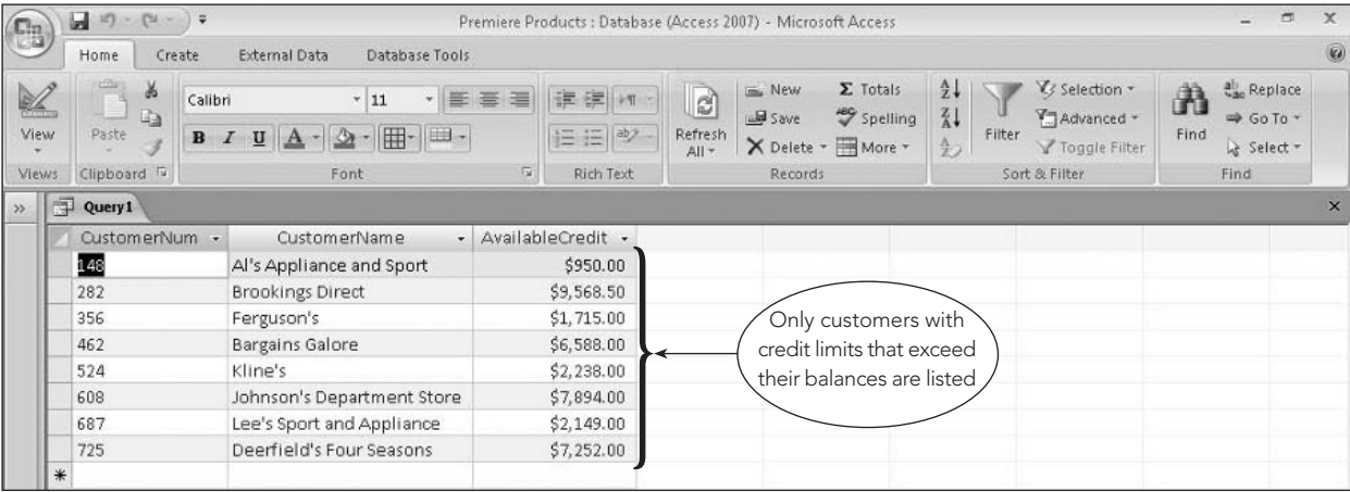
FIGURE 3-25 Query results
