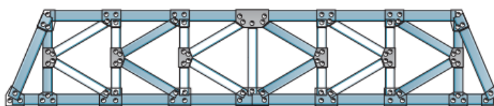
K-truss (g)
