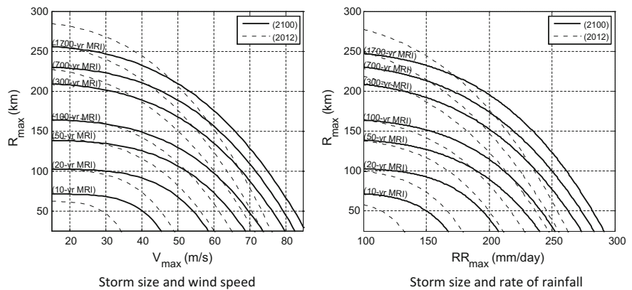
Fig. 6.6 Pairwise hazard curve examples, with and without impact of climate change. Source Authors own
