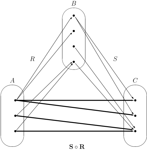
Figure 3.1 The composition S \circ R .
