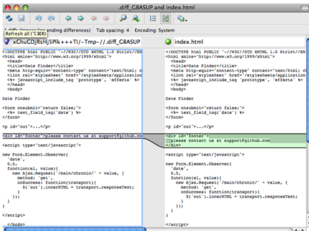
Figure 7.1: P4Merge.
