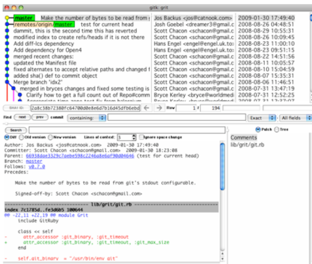
Figure 2.2: The gitk history visualizer.
