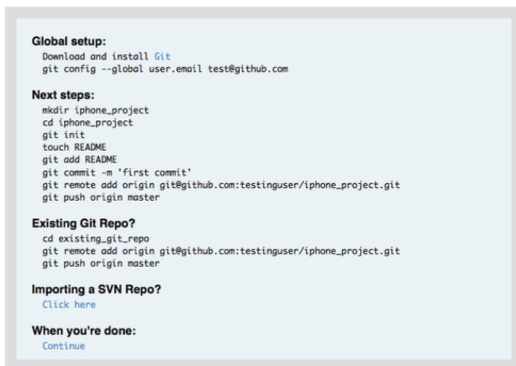
Figure 4.7: Instructions for a new repository.
