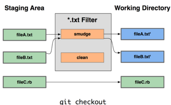
Figure 7.2: The “smudge” filter is run on checkout.
