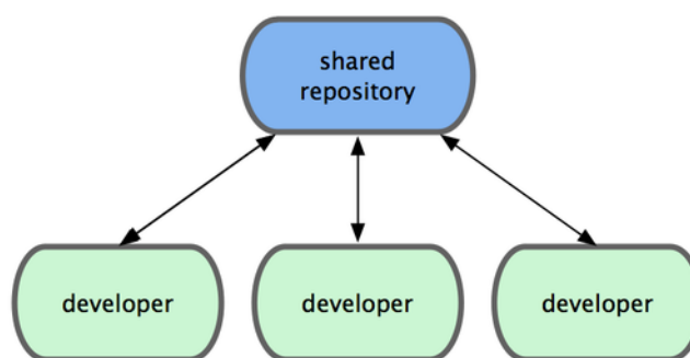
Figure 5.1: Centralized workflow.
