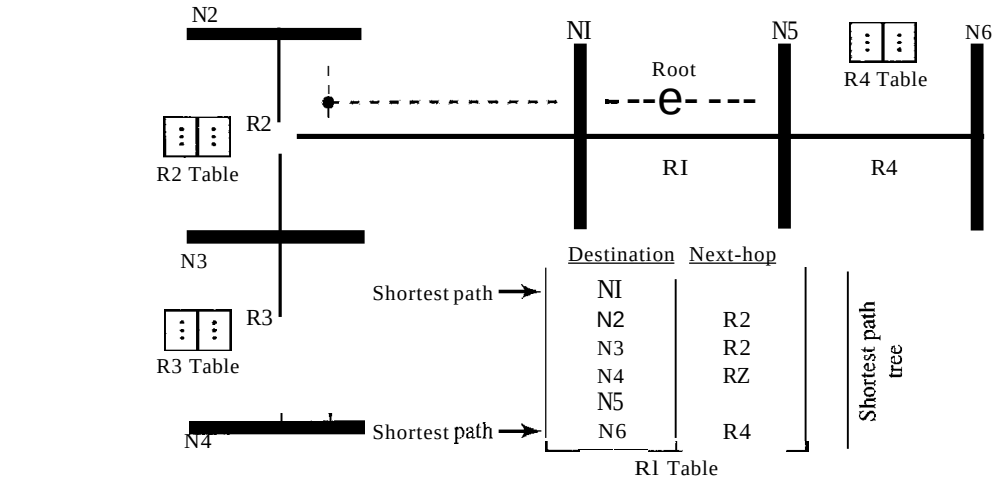
Figure 22.36 Shortest path tree in unicast routing
