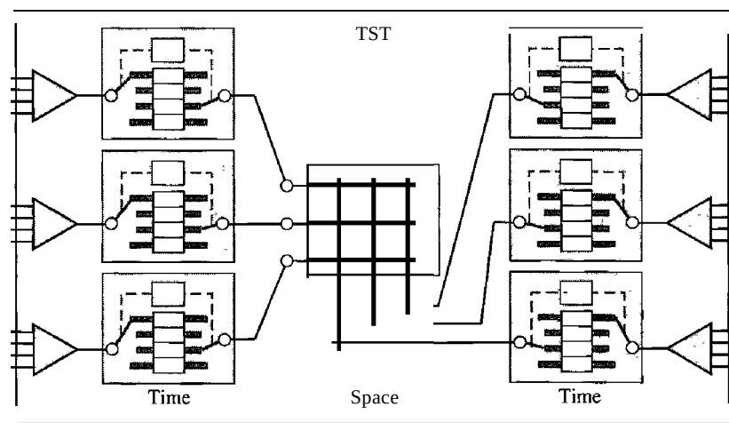
Figure 8.20 Time-space-time switch
