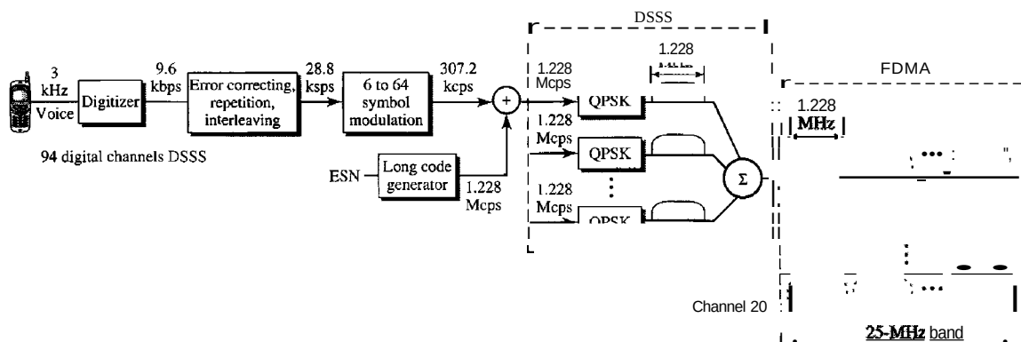
Figure 16.11 IS-95 reverse transmission
