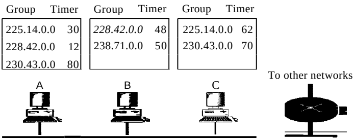
Figure 21.19 Example 21.6
