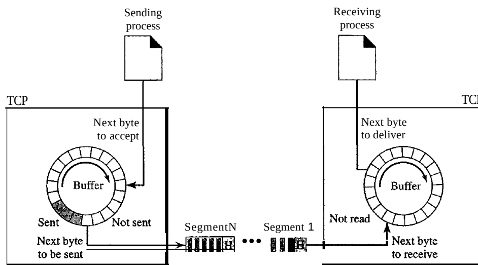
Figure 23.15 TCP segments
