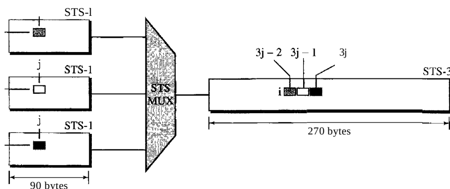
Figure 17.13 Byte interleaving
