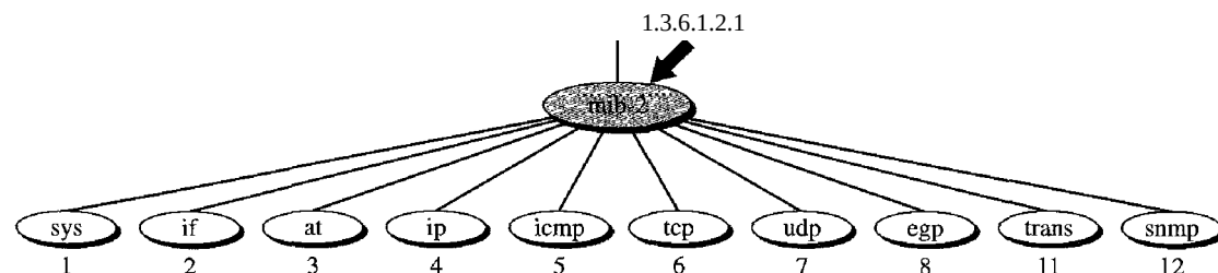
Figure 28.15 mib-2
