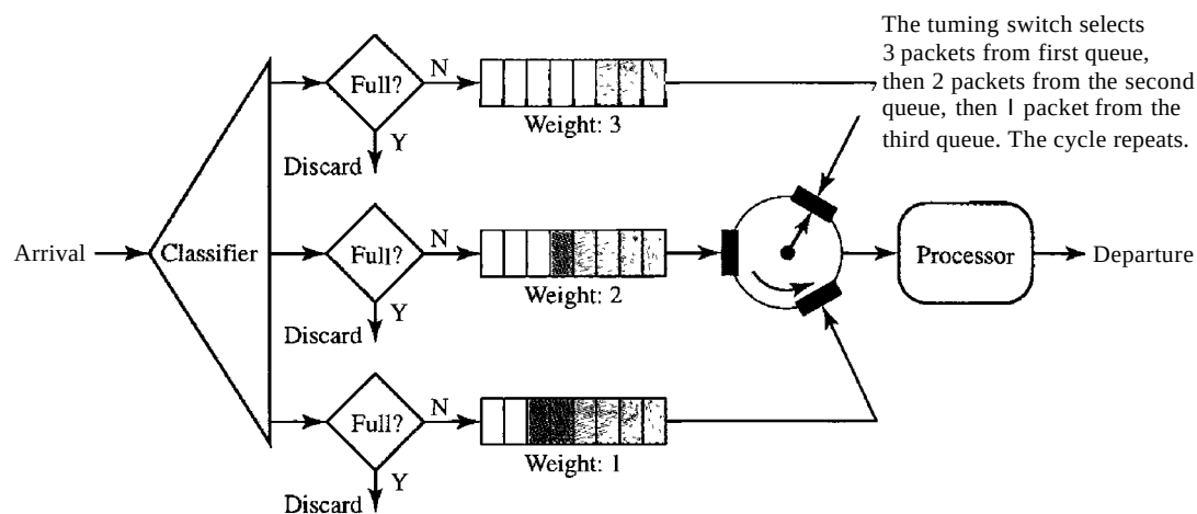
Figure 24.18 Weighted fair queuing
