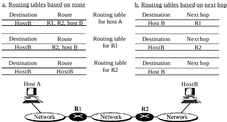
Figure 22.2 Route method versus next-hop method
