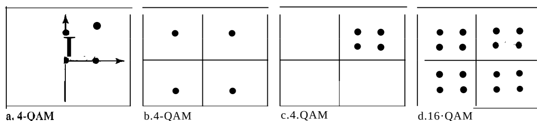
Figure 5.14 Constellation diagrams for some QAMs
