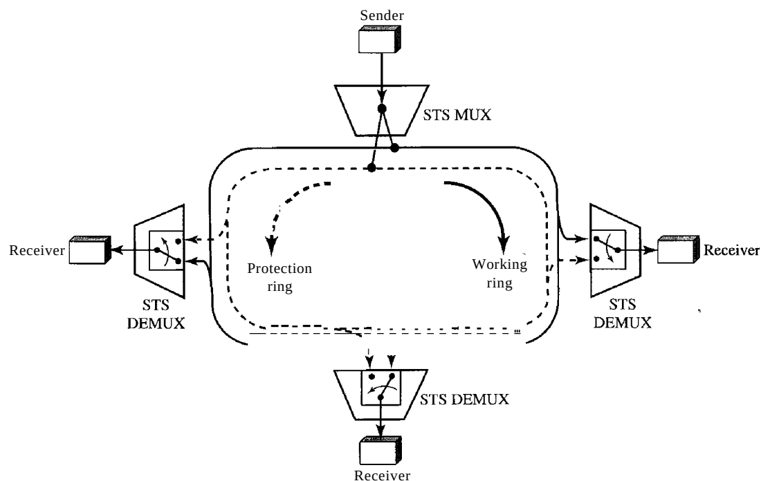
Figure 17.21 A unidirectional path switching ring
