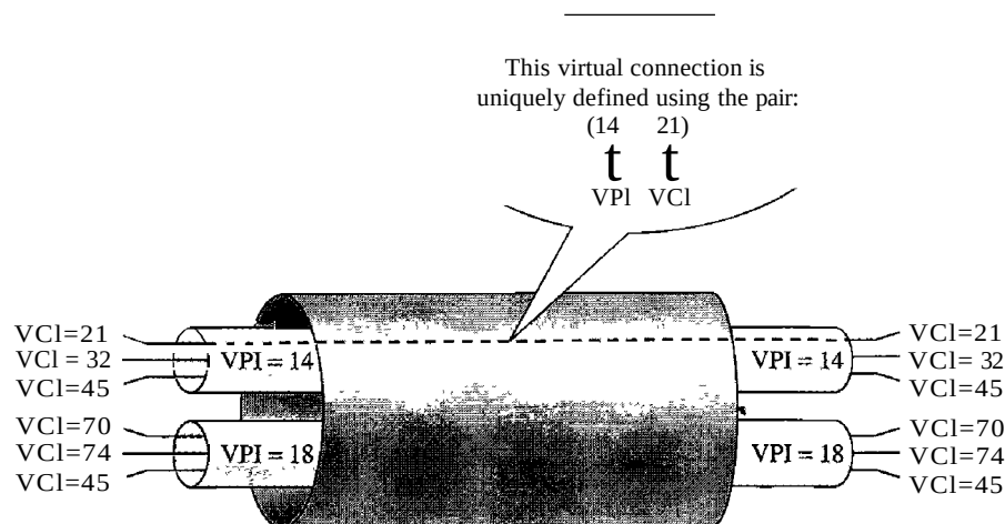
Figure 18.12 Connection identifiers
