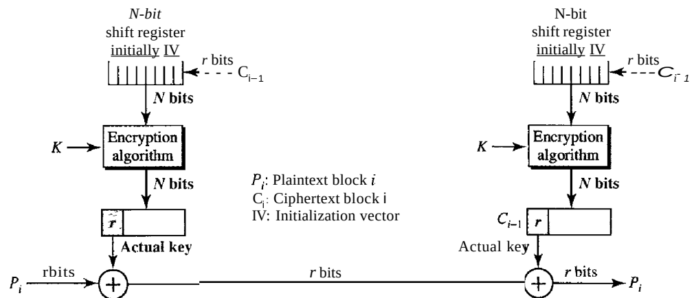
Figure 30.22 CFB mode
