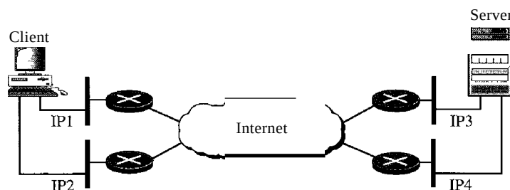
Figure 23.28 Multihoming concept
