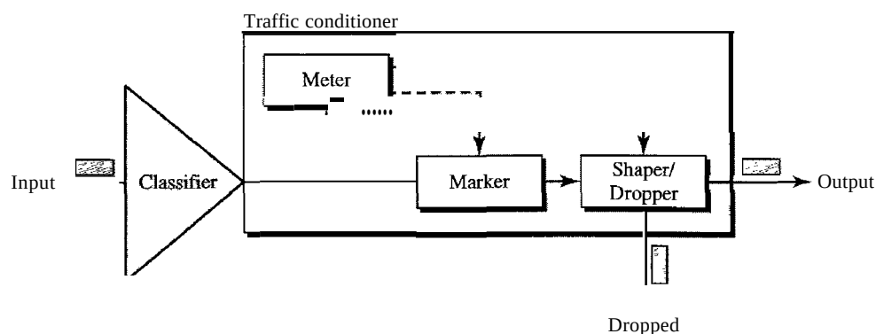
Figure 24.27 Traffic conditioner
