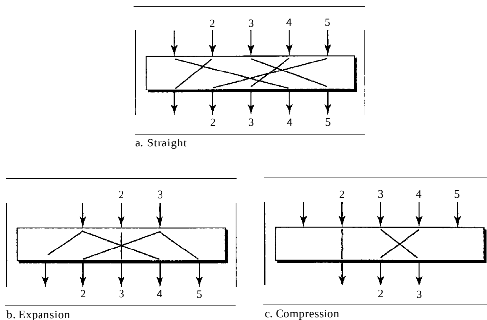
Figure 30.12 P-boxes: straight, expansion, and compression
