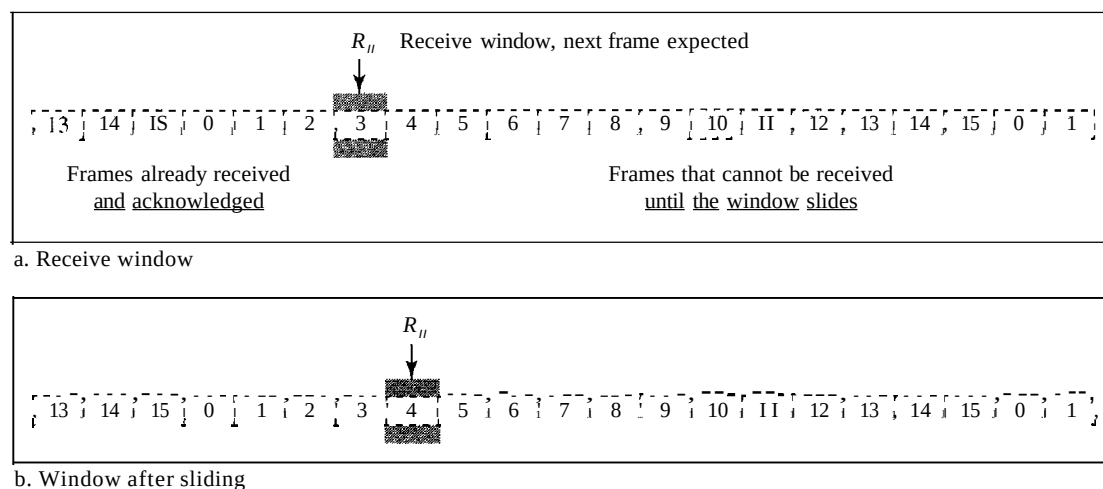
Figure 11.13 Receive window for Go-Back-NARQ
