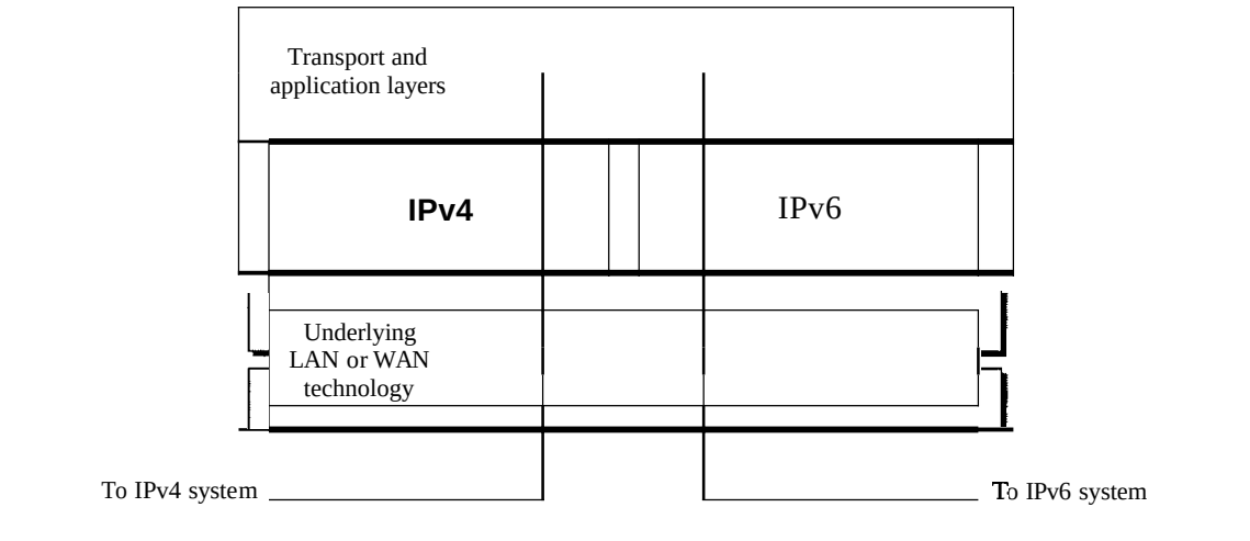
Figure 20.19 Dual stack
