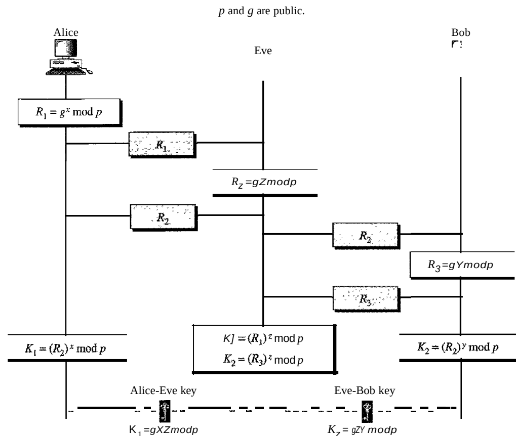
Figure 30.28 Man-in-the-middle attack
