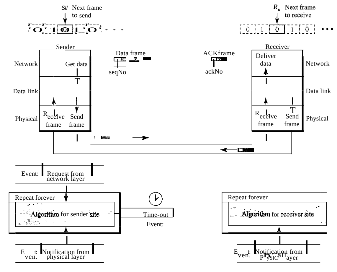
Figure 11.10 Design of the Stop-and-Wait ARQ Protocol
