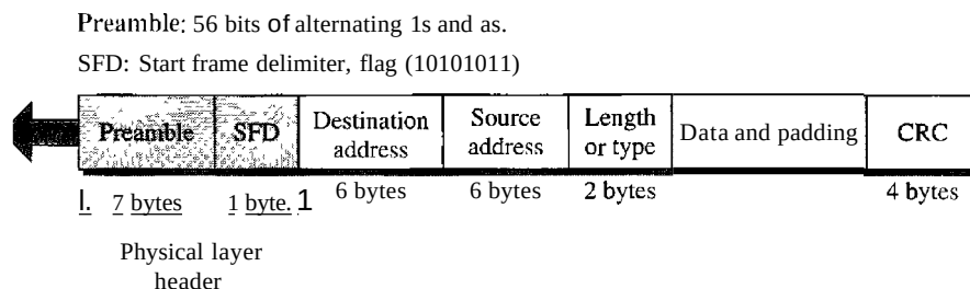
Figure 13.4 802.3 MAC frame
