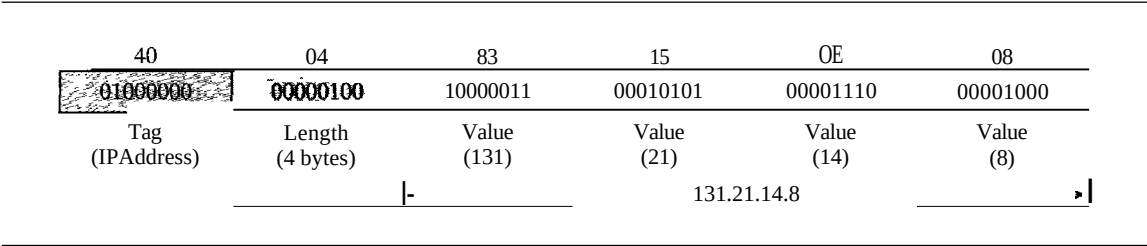
Figure 28.14 Example 28.4, IPAddress 131.21.14.8
