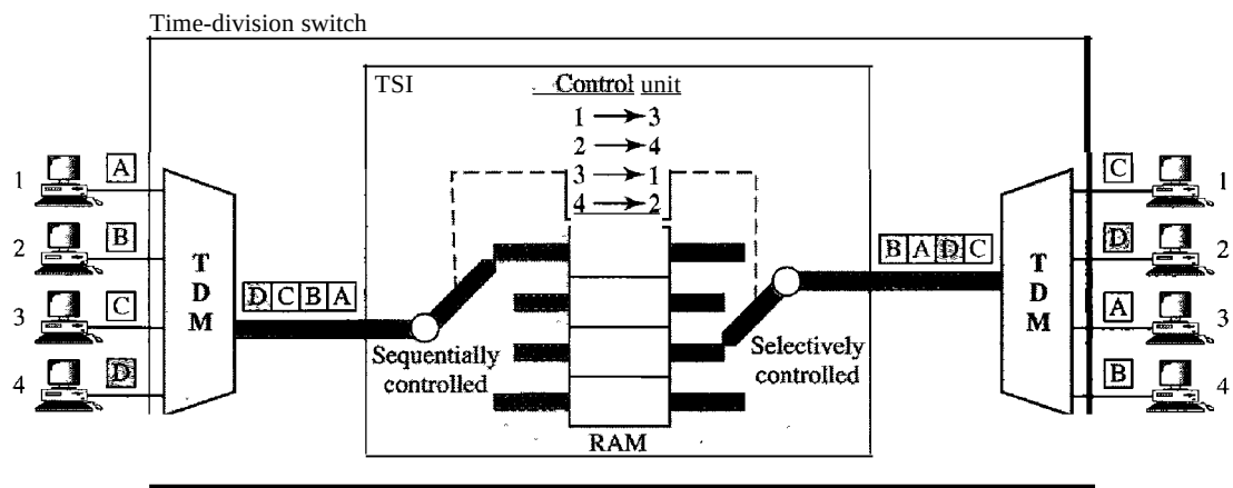
Figure 8.19 Time-slot interchange
