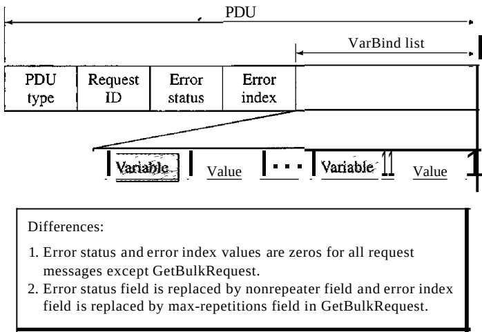
Figure 28.21 SNMP PDUformat
