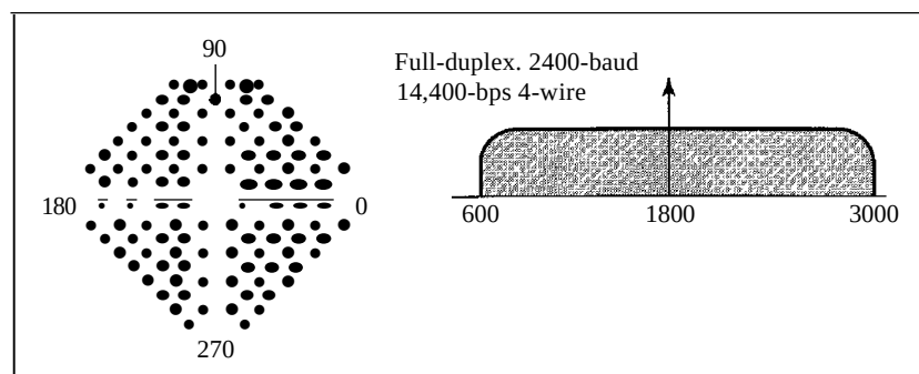
b. Constellation and bandwidth for V.32bis
