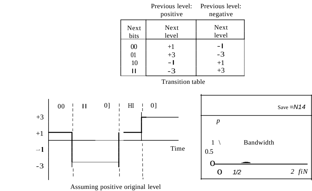
Figure 4.10 Multilevel: 2B1Q scheme
