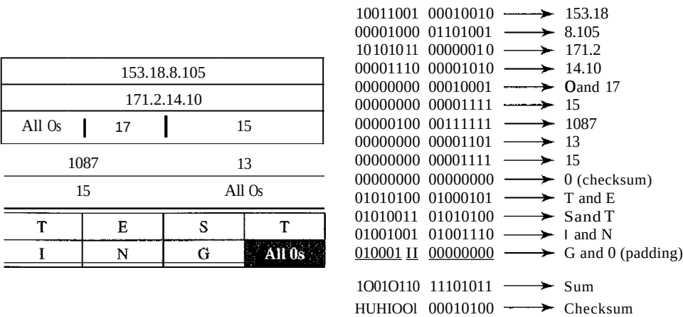
Figure 23.11 Checksum calculation of a simple UDP user datagram
