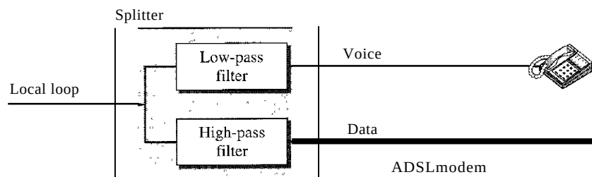
Figure 9.12 ADSL modem
