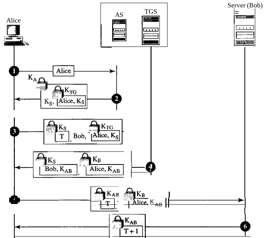
Figure 31.22 Kerberos example
