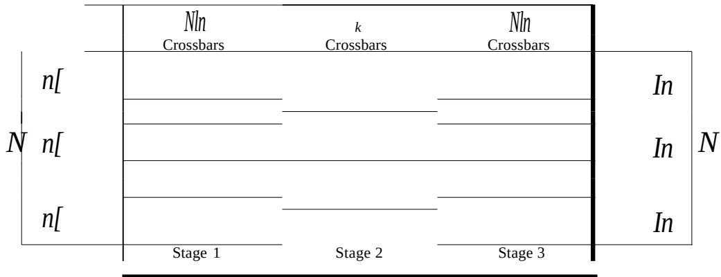
Figure 8.18 Multistage switch
