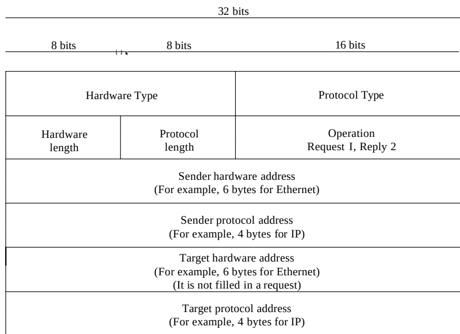
Figure 21.2 ARP packet
