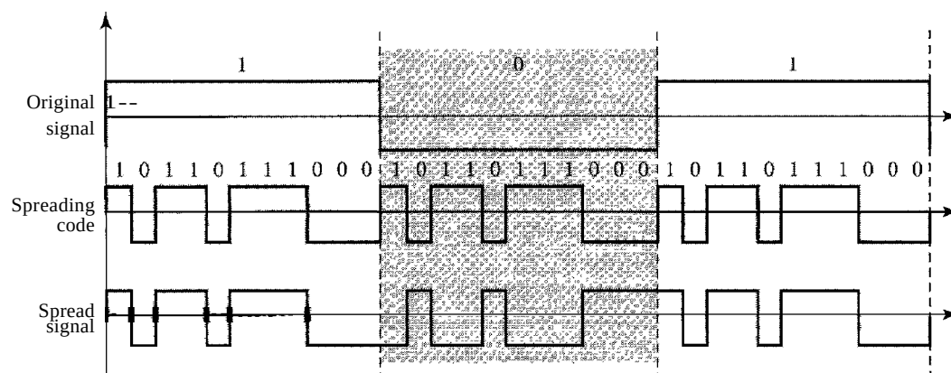
Figure 6.33 DSSS example
