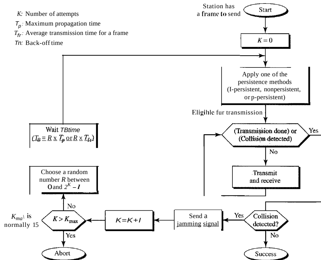
Figure 12.14 Flow diagram for the CSMA/CD
