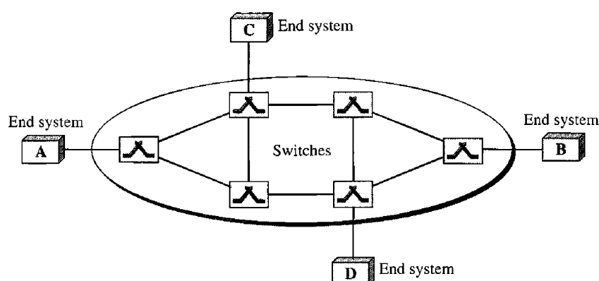
Figure 8.10 Virtual-circuit network
