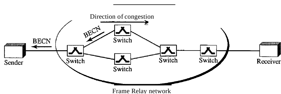
Figure 24.12 BECN
