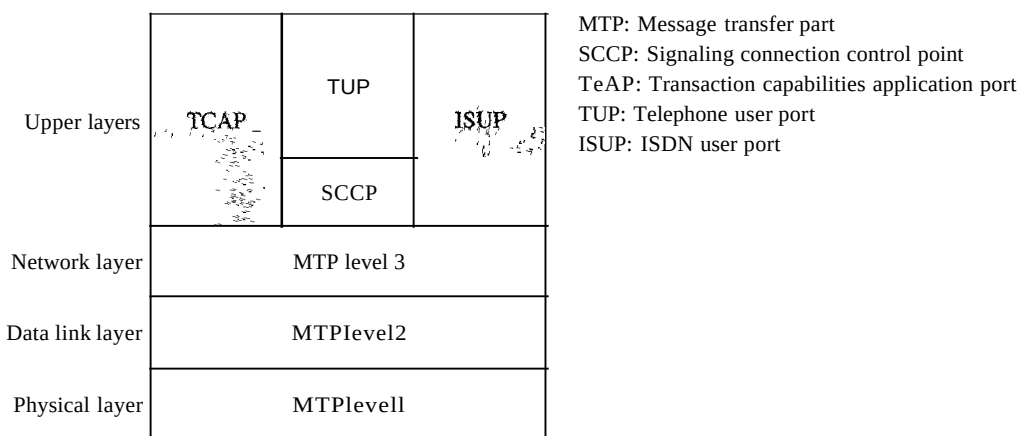
Figure 9.5 Layers in SS7
