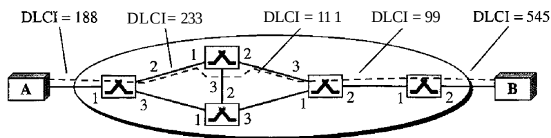
Figure 18.31 Exercise 18
