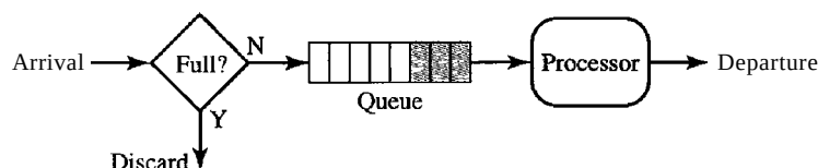
Figure 24.16 FIFO queue
