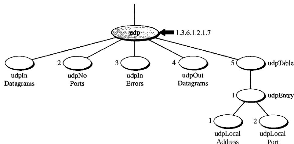
Figure 28.16 udp group
