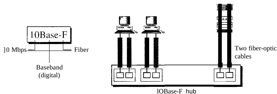
Figure 13.13 IOBase-F implementation
