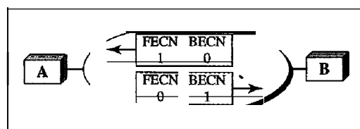
c. Congestion in the direction B-A
