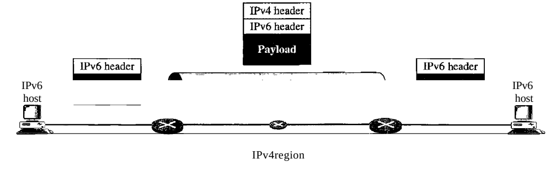
Figure 20.20 Tunneling strategy
