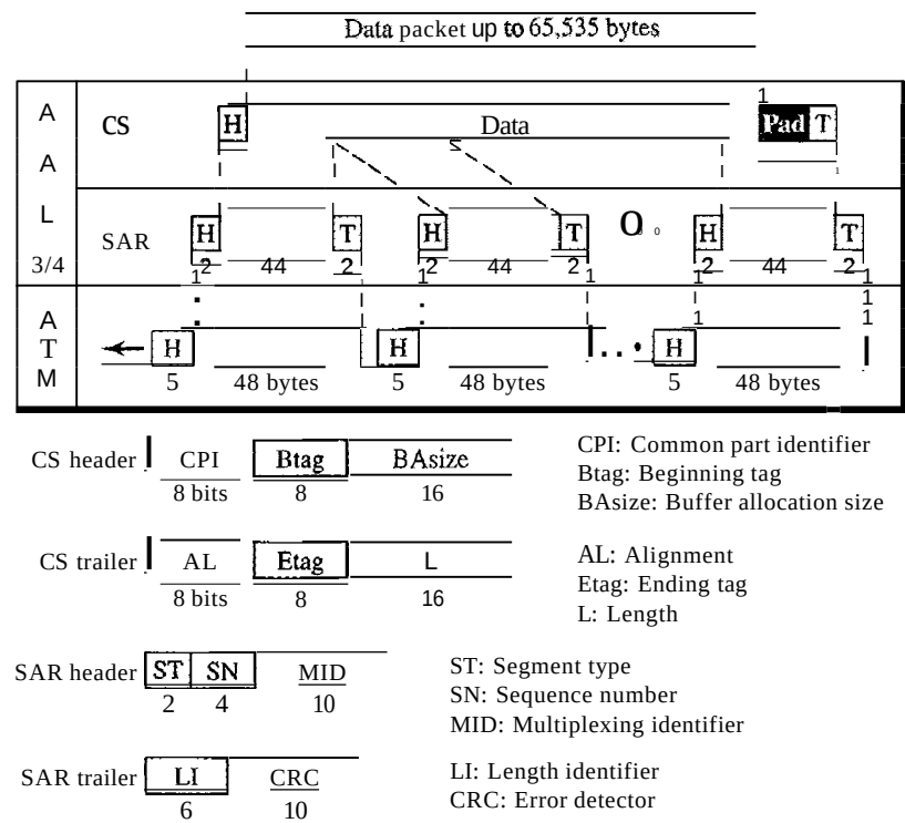
Figure 18.22 AAL3/4
