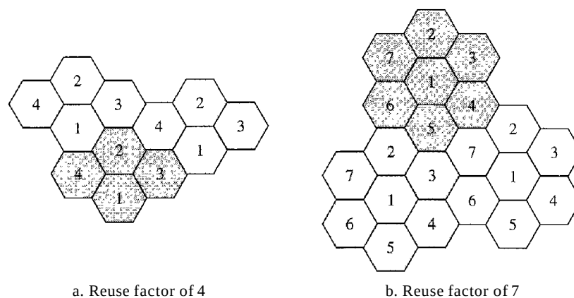
Figure 16.2 Frequency reuse patterns
