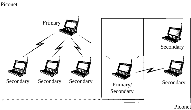
Figure 14.20 Scatternet
