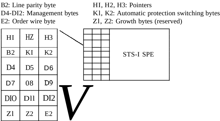
Figure 17.8 STS-I frame: line overhead
