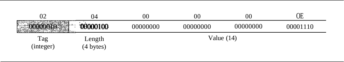
Figure 28.11 Example 28.1, INTEGER 14
