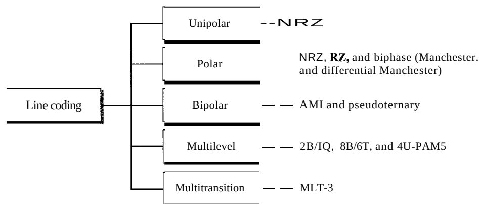
Figure 4.4 Line coding schemes
