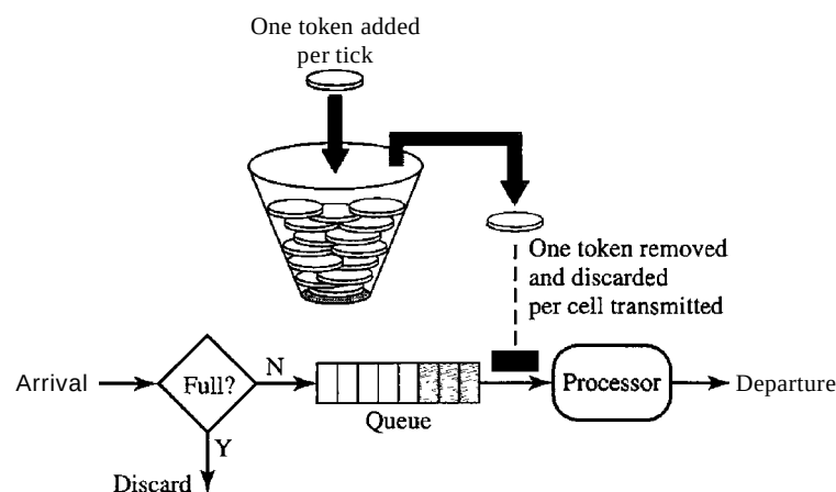
Figure 24.21 Token bucket
