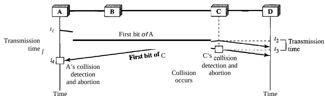
Figure 12.12 Collision of the first bit in CSMA/CD
