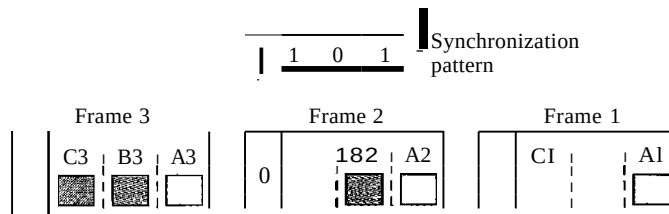
Figure 6.22 Framing bits
