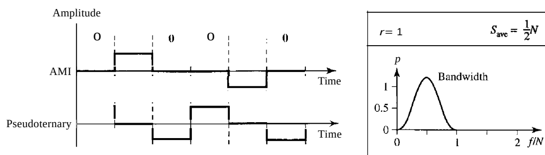
Figure 4.9 Bipolar schemes: AMI and pseudoternary
