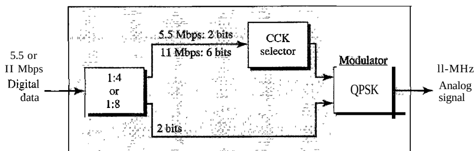
Figure 14.18 Physical layer of IEEE 802.11b
