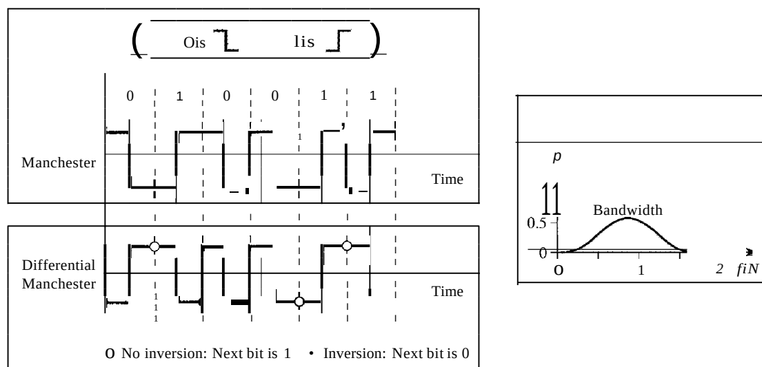
Figure 4.8 Polar biphase: Manchester and differential Manchester schemes
