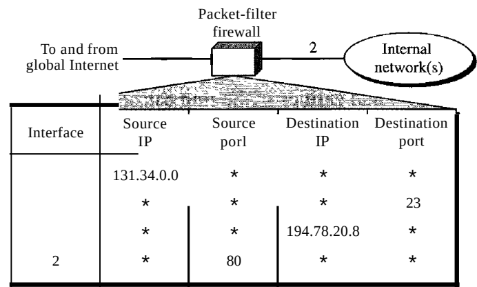
Figure 32.23 Packet-filter firewall
