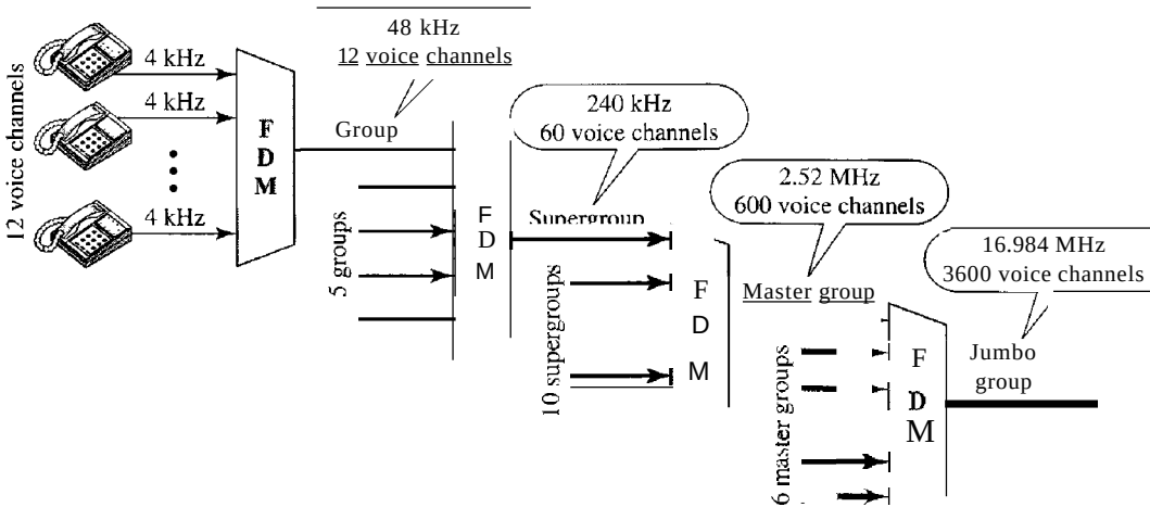
Figure 6.9 Analog hierarchy
