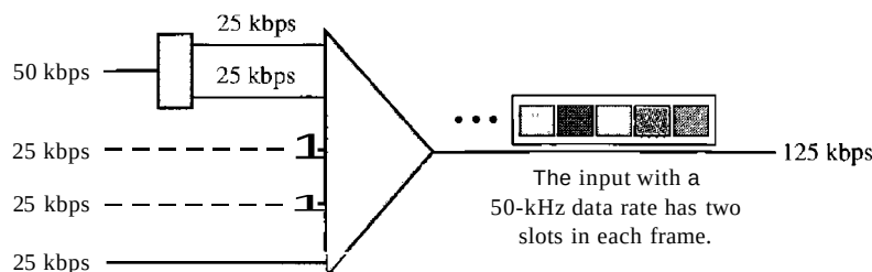
Figure 6.20 Multiple-slot multiplexing
