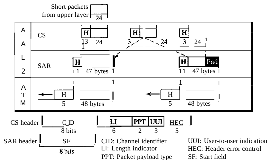
Figure 18.21 AAL2
