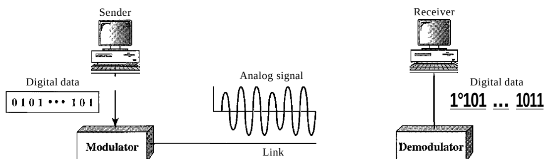
Figure 5.1 Digital-to-analog conversion
