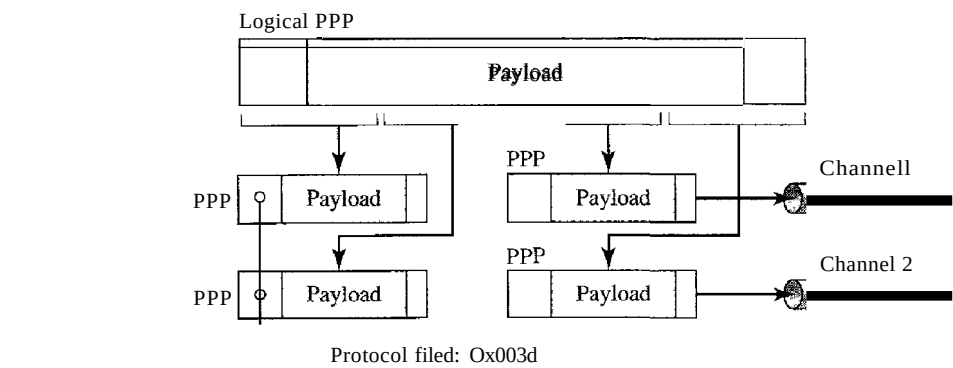
Figure 11.40 Multilink PPP
