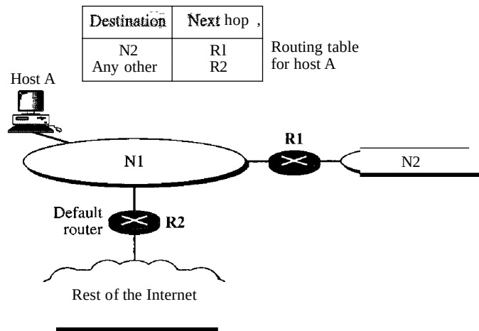
Figure 22.4 Default method
