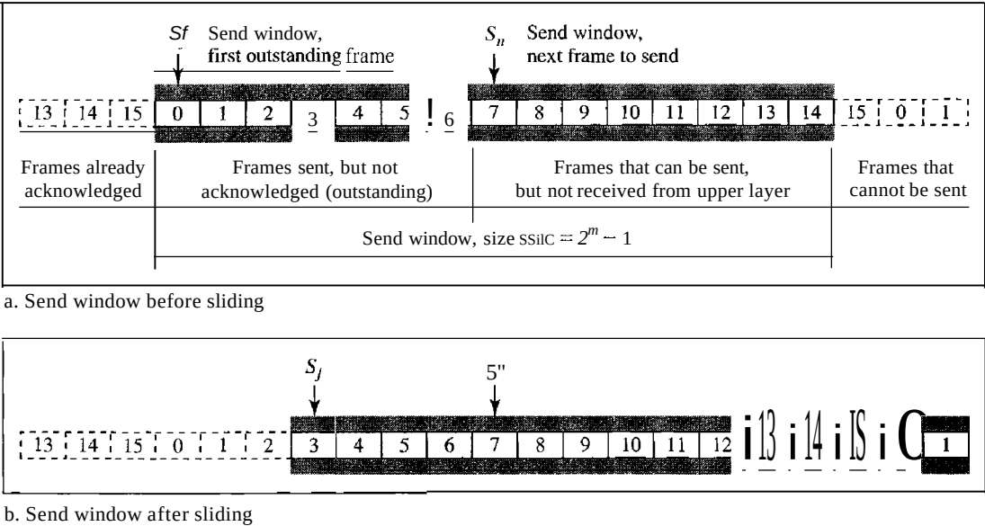
Figure 11.12 Send window for Go-Back-NARQ
