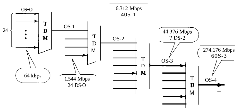
Figure 6.23 Digital hierarchy
