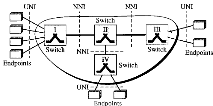
Figure 18.9 Architecture of an ATM network
