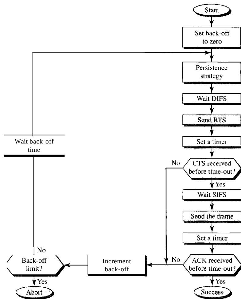
Figure 14.4 CSMA/CA flowchart
