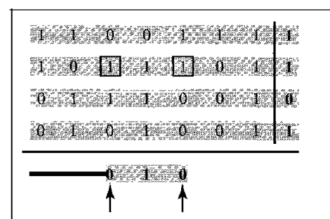
c. Two errors affect two parities
