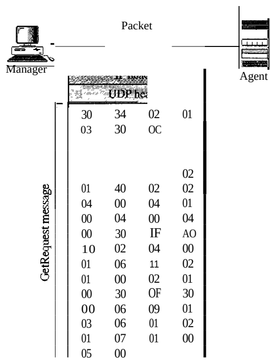
Figure 28.24 GetRequest message
