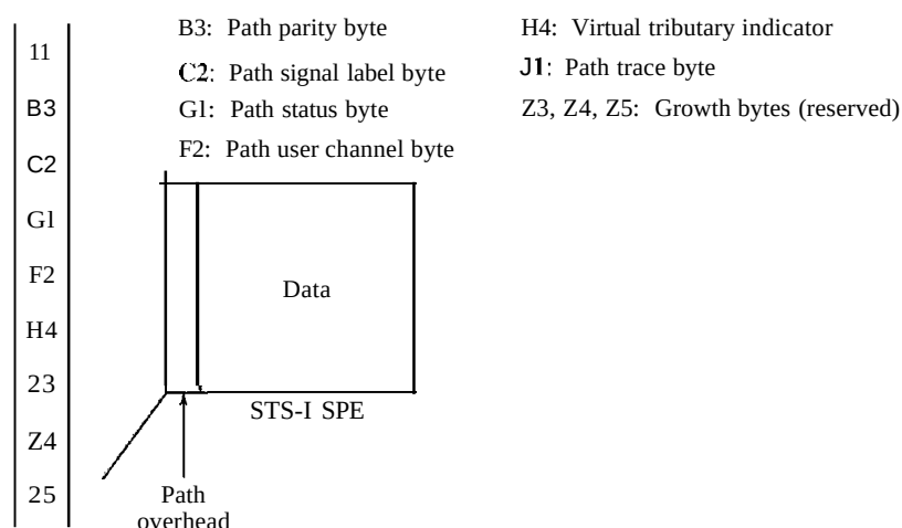
Figure 17.9 STS-1 frame: path overhead
