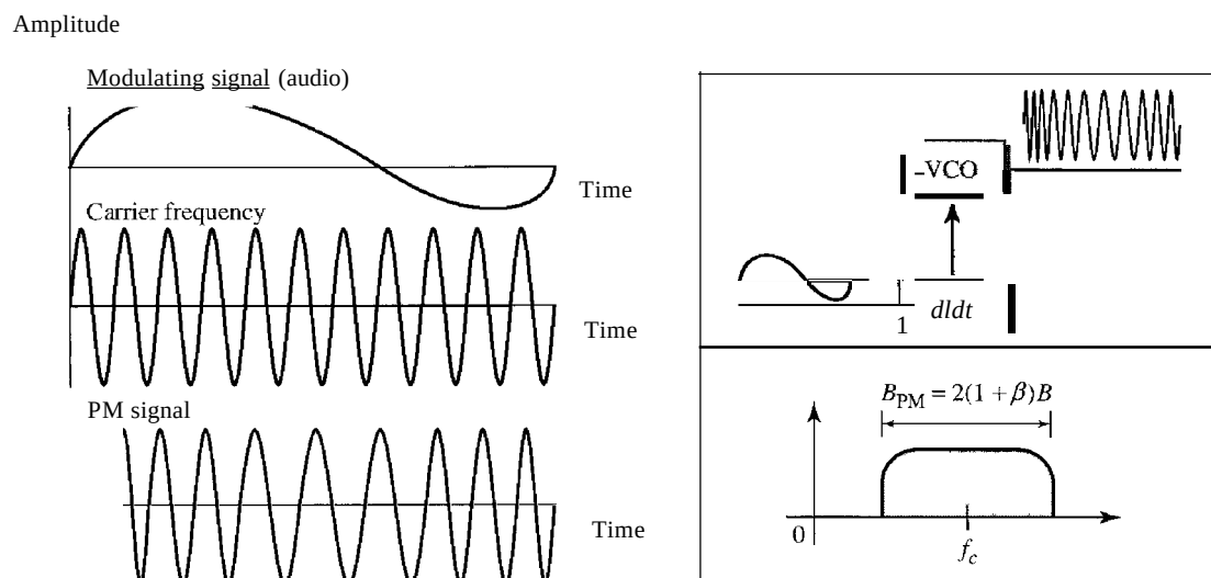
Figure 5.20 Phase modulation
