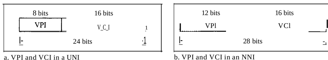
Figure 18.13 Virtual connection identifiers in UNIs and NNIs
