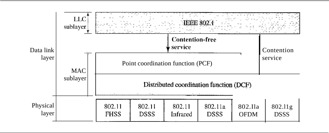
Figure 14.3 MAC layers in IEEE 802.11 standard
