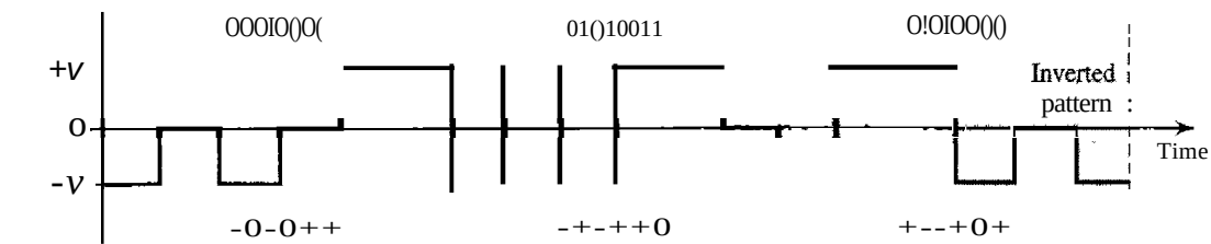
Figure 4.11 Multilevel: 8B6T scheme
