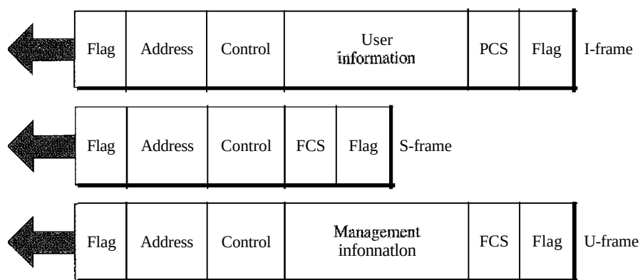
Figure 11.27 HDLC frames
