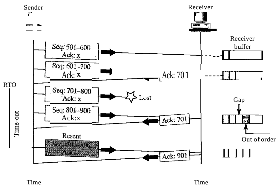
Figure 23.25 Lost segment
