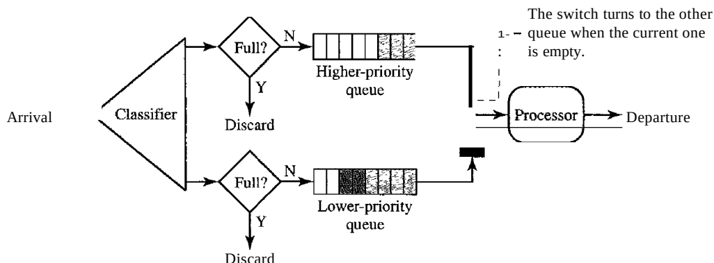
Figure 24.17 Priority queuing
