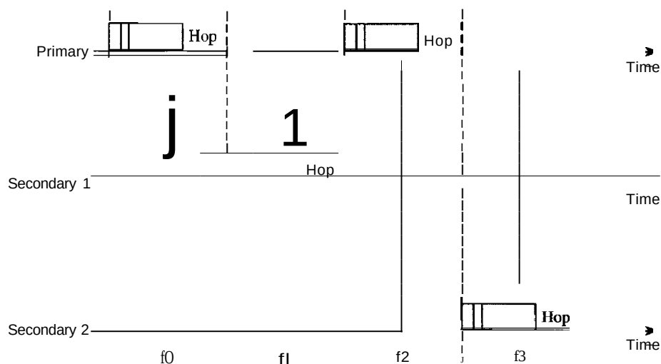
Figure 14.23 Multiple-secondary communication
