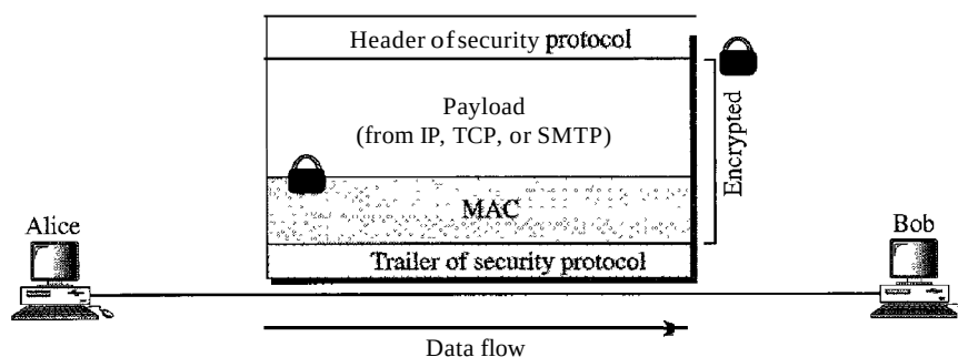
Figure 32.1 Common structure of three security protocols
