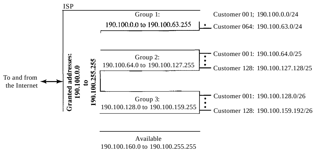
Figure 19.9 An example of address allocation and distribution by an IS?
