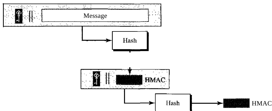
Figure 31.10 HMAC
