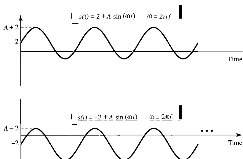
Figure C.3 Vertical shifting of sine waves
