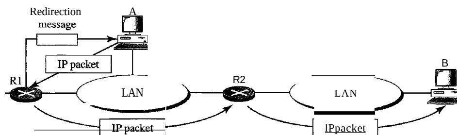
Figure 21.11 Redirection concept
