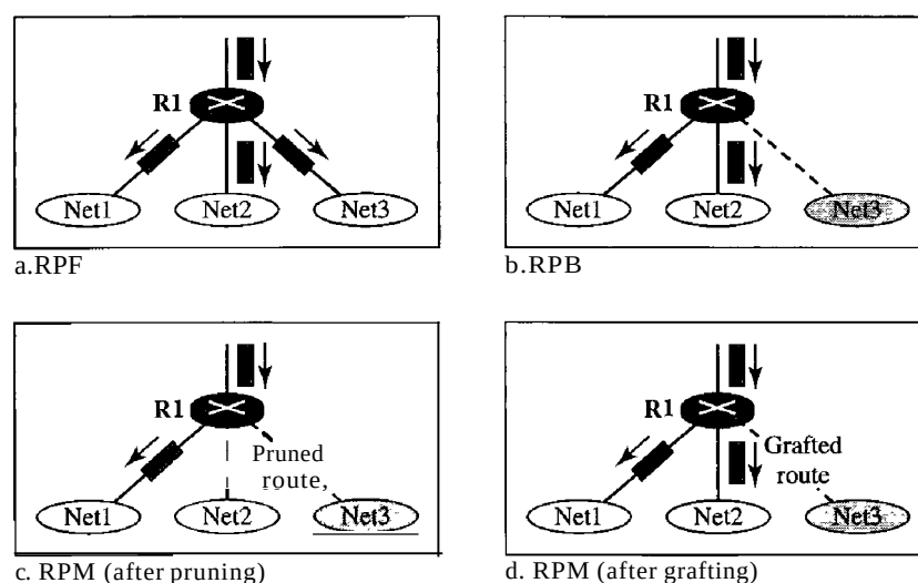
Figure 22.43 RPF, RPB, and RPM
