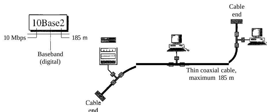
Figure 13.11 10Base2 implementation
