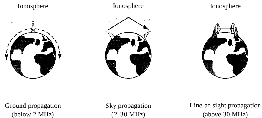
Figure 7.18 Propagation methods
