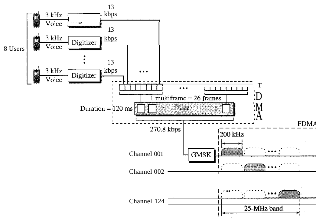
Figure 16.8 GSM
