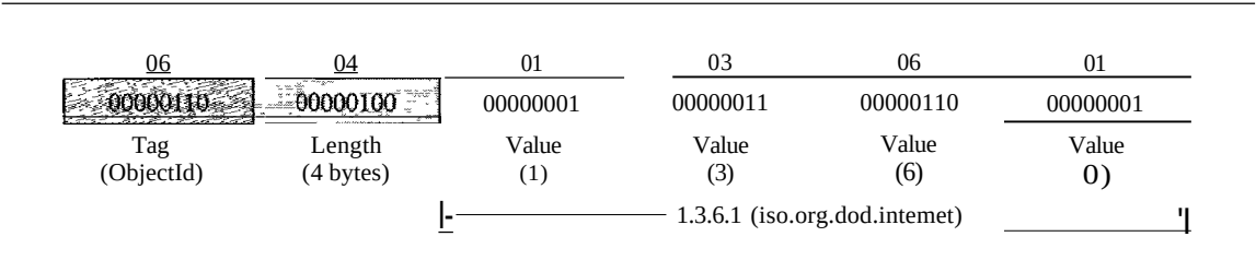
Figure 28.13 Example 28.3, ObjectIdentifier 1.3.6.1
