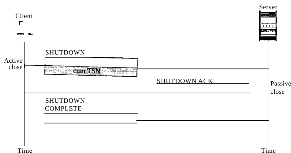
Figure 23.35 Association termination
