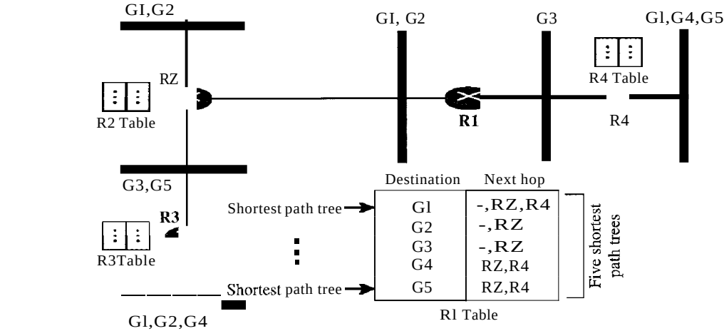
Figure 22.37 Source-based tree approach
