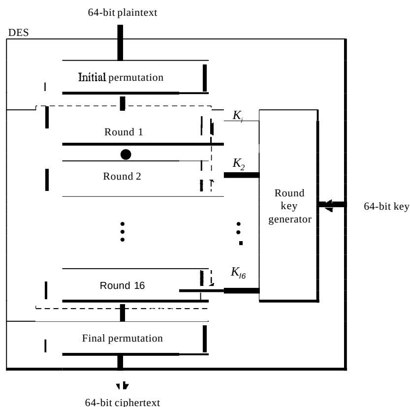
Figure 30.13 DES
