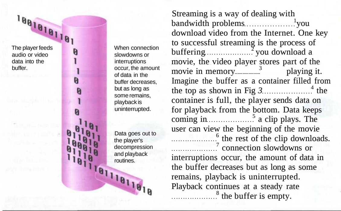
Fig 3 Video buffering
