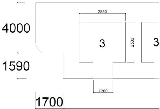
Fragment plan of the Buddhist temple
