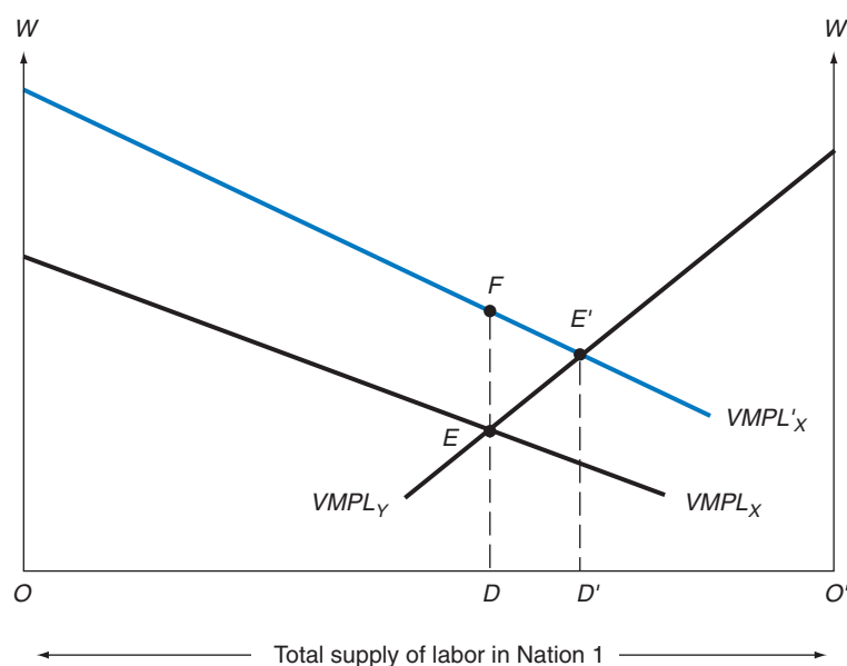
FIGURE 5.9. Specific-Factors Model.
