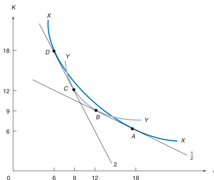
FIGURE 5.10. Factor-Intensity Reversal.
