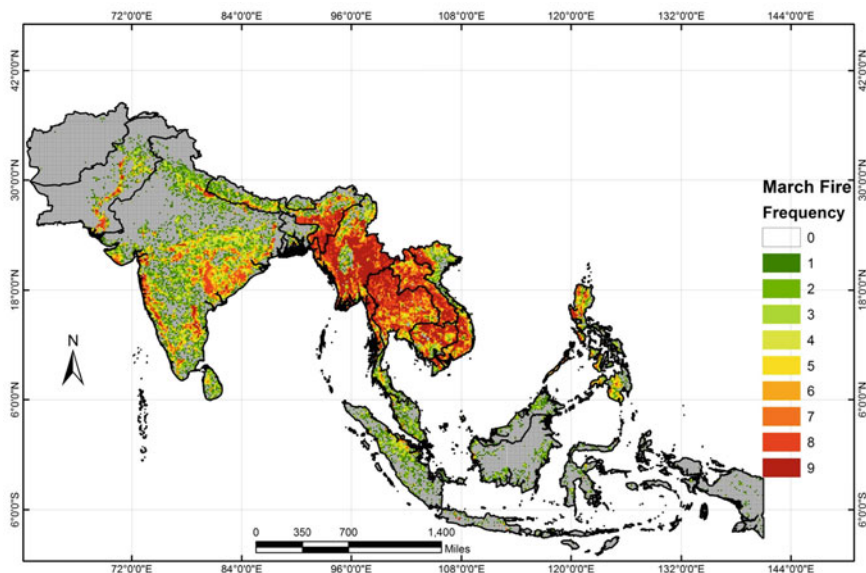
Fig. 5 Fire frequency per 9.3 \text{ km}^2 grid cells during the month of March (2003–2011)
