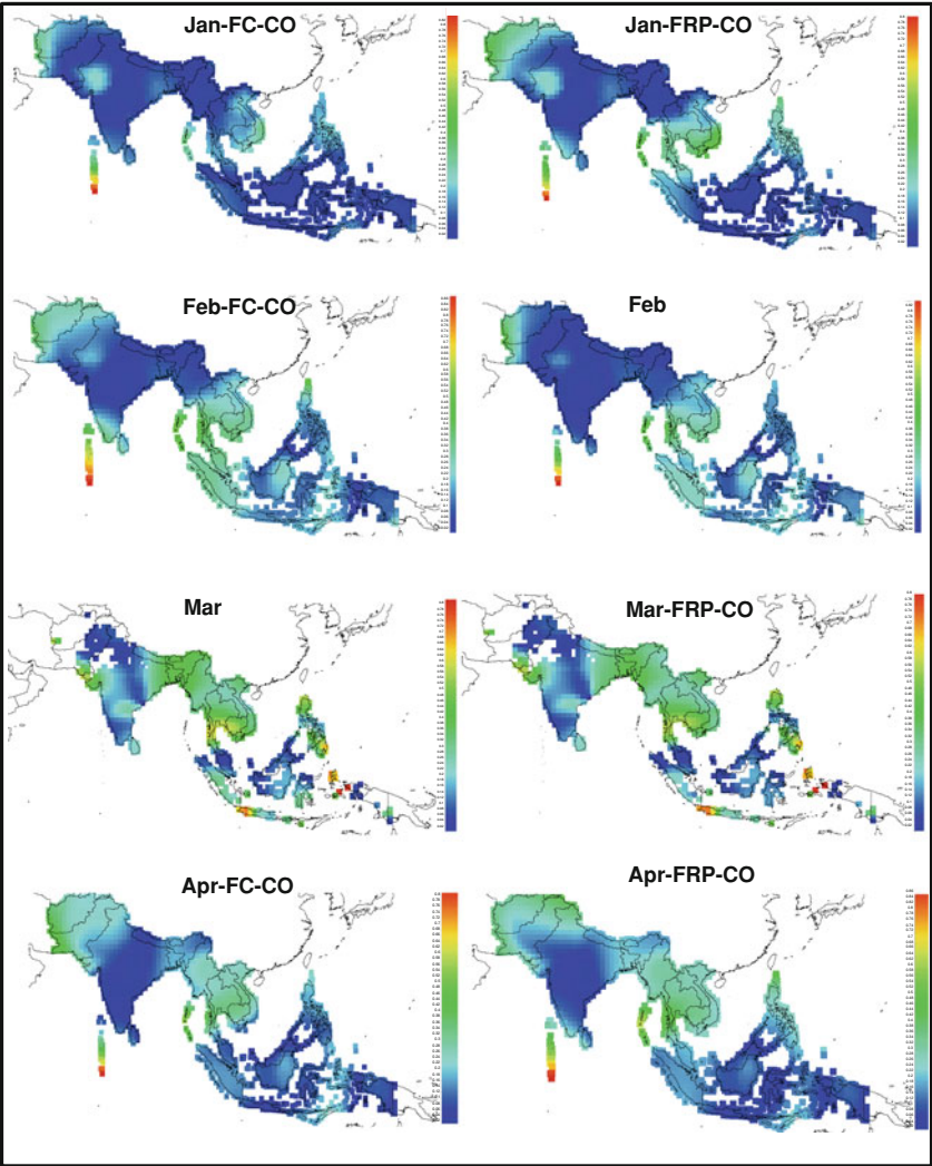
Fig. 9 a Spatial correlations between MODIS fire counts (FC), FRP and CO for individual months at 0.5 \times 0.5 degree grid cells. b The correlation values from ordinary least square regression (OLR) and local regression are shown in Table 3
