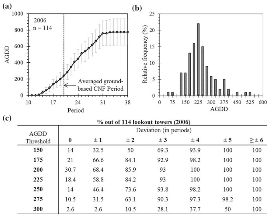
Fig. 2 Determination of AGDD threshold for CNF occurrence: a averaged temporal trends of AGDD at all of the lookout tower sites during 2006, and the dotted vertical line shows the averaged ground-based CNF observation period; b relative frequency of the AGDD at all of lookout tower sites; and c implementation of various AGDD threshold to determine the best threshold in predicting the CNF period
