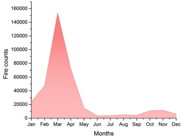
Fig. 3 MODIS aqua and terra monthly fire counts (averaged from 2002–2012)
