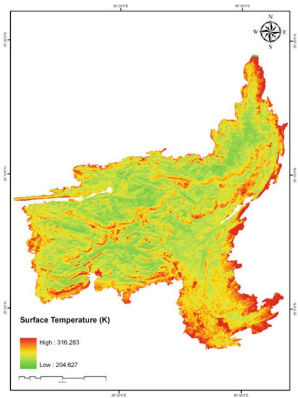
Fig. 5 Land surface temperature (LST) in Kelvin
